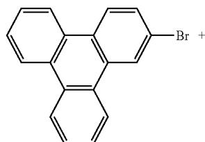
[Reaction Scheme 13]
