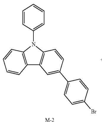
[Reaction Scheme 11]
