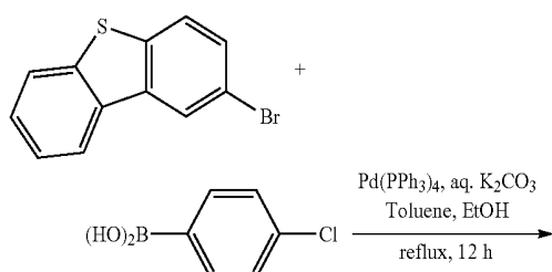
[Reaction Scheme 10]
