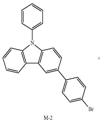
[Reaction Scheme 12]
