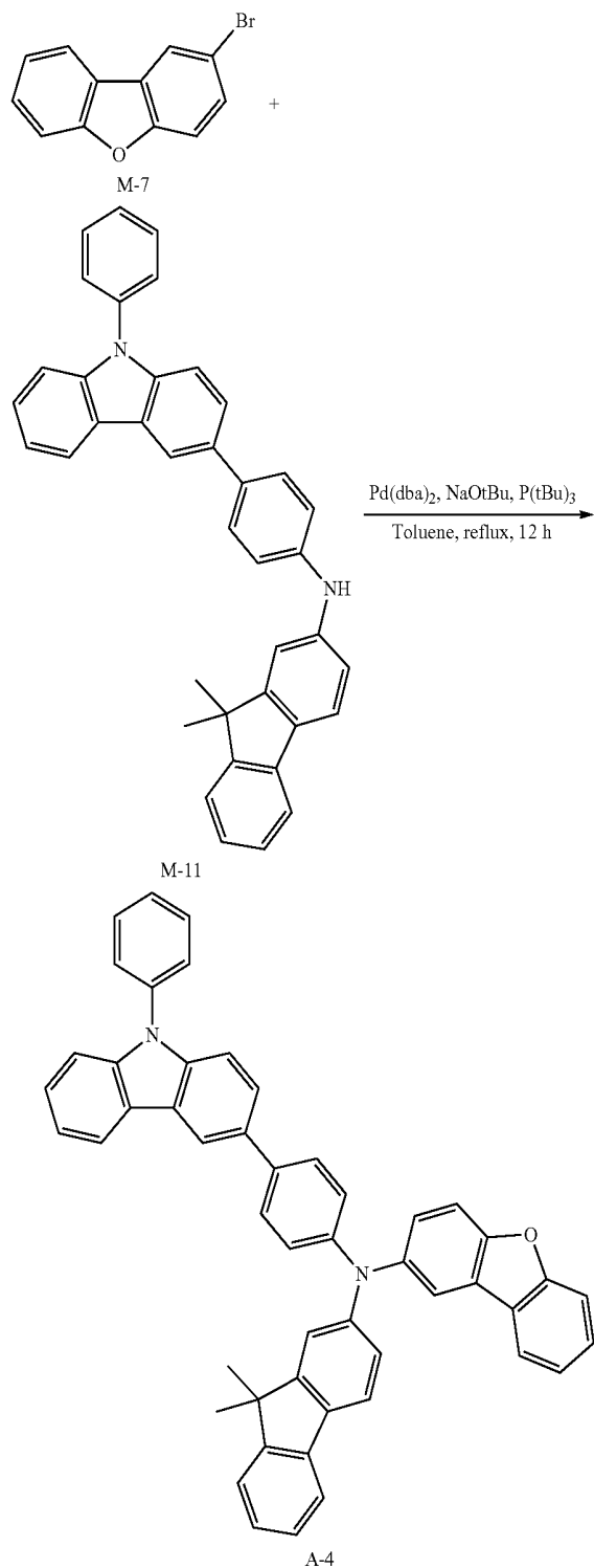
[Reaction Scheme 16]
