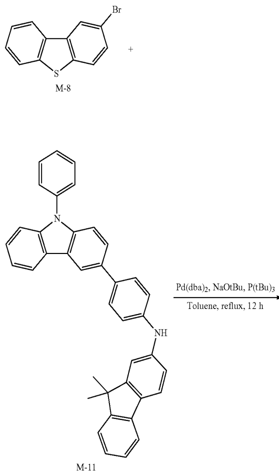
[Reaction Scheme 17]
