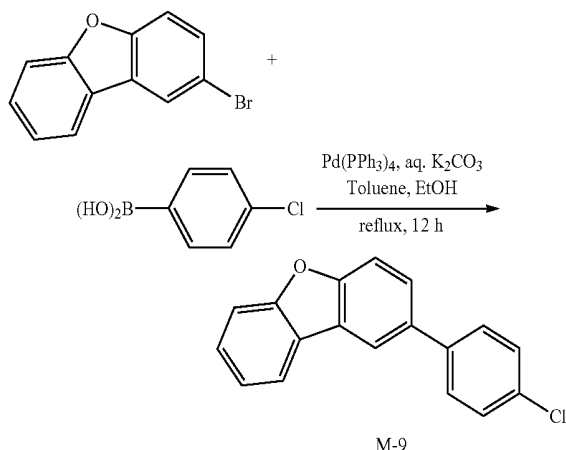
[Reaction Scheme 9]
